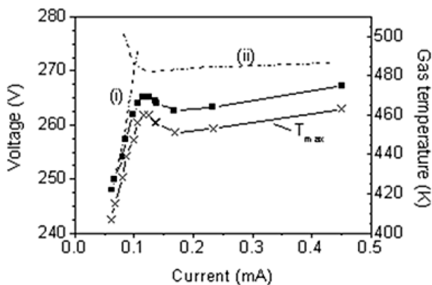
Fig. 15. Calculated V - I characteristic (■) and peak gas temperature (x) vs. current (Xe, 100 Torr; D = 280 \mu\text{m} ). The dashed lines (i) and (ii) are characteristics calculated for discharges sustained by electron emission from inside the hollow cathode or from the outer surface of the cathode, respectively [51].
