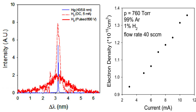
Fig. 27. Left: stark-broadened profile of the Balmer H_\beta line at 486.1 nm for dc and pulsed (10 ns) operation. Also shown is the apparatus profile using the Hg 435.8 nm line. Right: electron density of a 1 atm dc Ar MHC discharge vs. discharge current [83].
