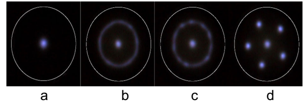
Fig. 6. (a) Single plasma spot observed at a Xe pressure of 50 Torr and 0.05 mA; (b) target shape plasma pattern at 100 Torr and 0.132 mA; (c) target shape plasma pattern with clear nodes at 100 Torr and 0.137 mA, and (d) six plasma spots observed at 100 Torr and 0.136 mA [38].
