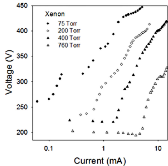
Fig. 7. V - I characteristics of Xe CBL discharges at various pressures. The cathode opening is 1.5 mm in diameter [36].
