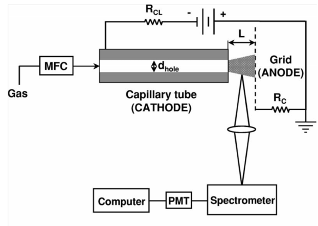
Fig. 17. Schematic diagram of a hollow cathode plasma microjet with optical emission spectroscopy setup [55].
