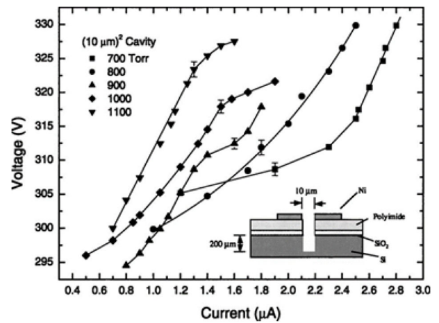
Fig. 16. V - I characteristics of 10 \mu\text{m} silicon trench micro-cathode devices operating in neon at various pressures. The inset shows a generalized schematic diagram of the device structure [53].
