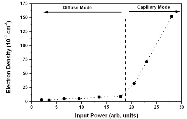
Fig. 23. Electron density in a He CPE discharge as a function of power input. The transition of the discharge from the diffuse to the capillary mode with a concurrent drastic increase in the electron density is clearly apparent [72].
