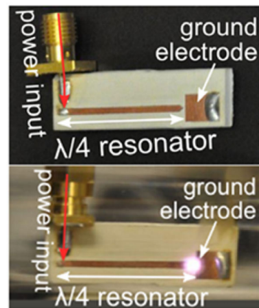
Fig. 10. Photographs of a 1 GHz quarter-wave generator show a 20 mm long microstrip device with (bottom) and without (top) a microplasma [12].
